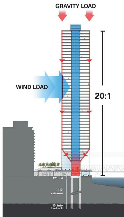
BUILDING SECTION
